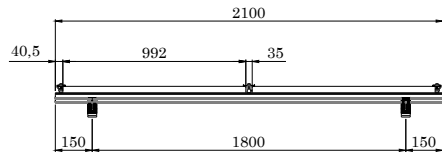
VISTA FRONTAL
